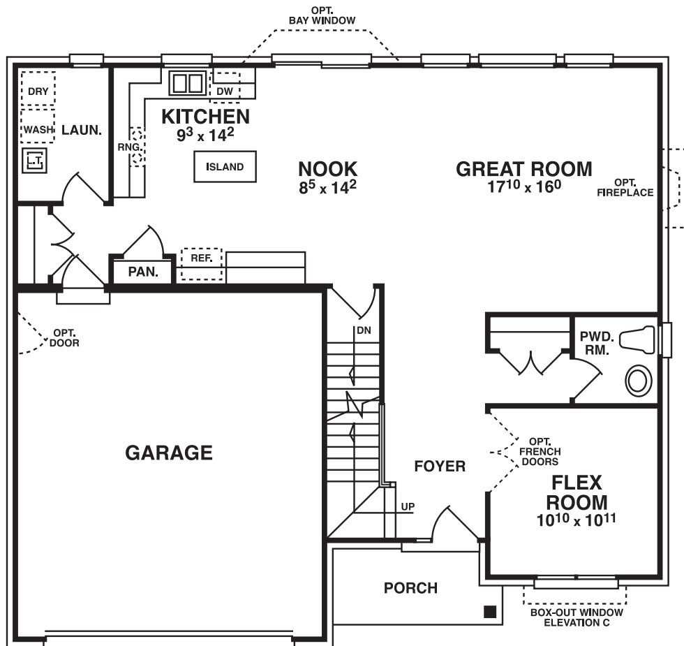
FIRST FLOOR PLAN ELEVATION C
