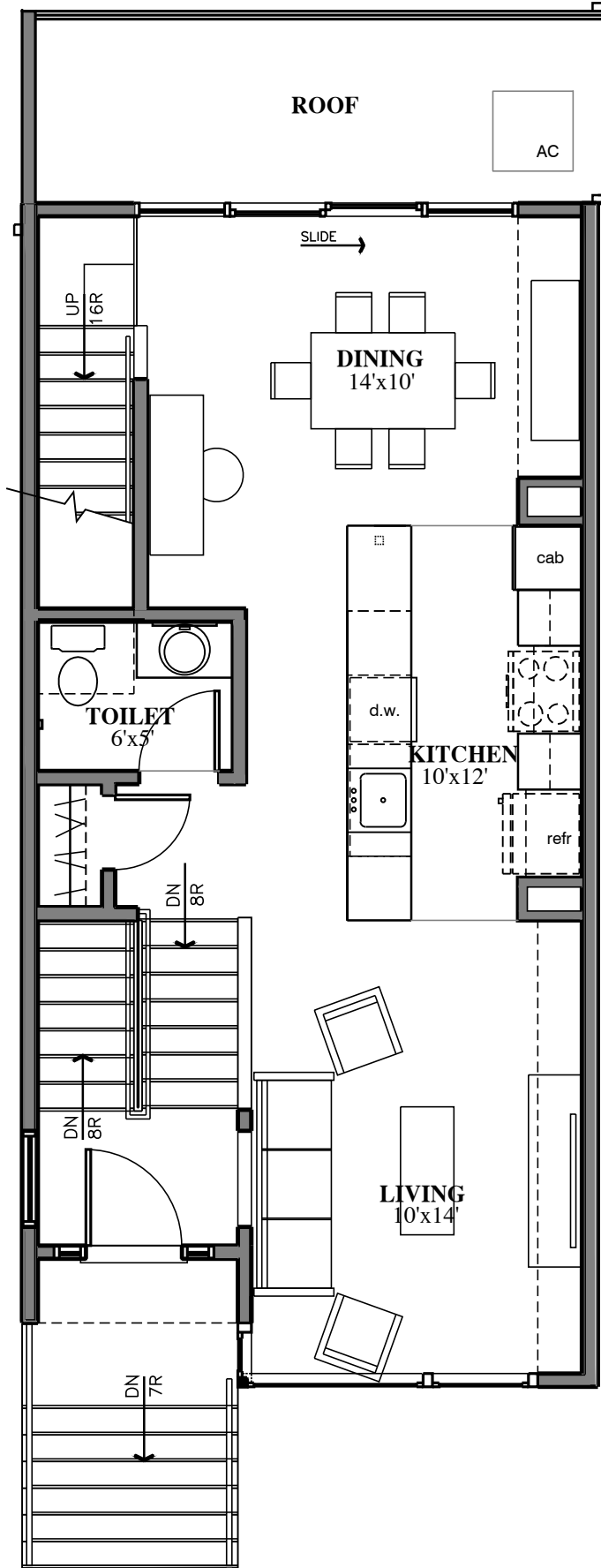
MAIN FLOOR
