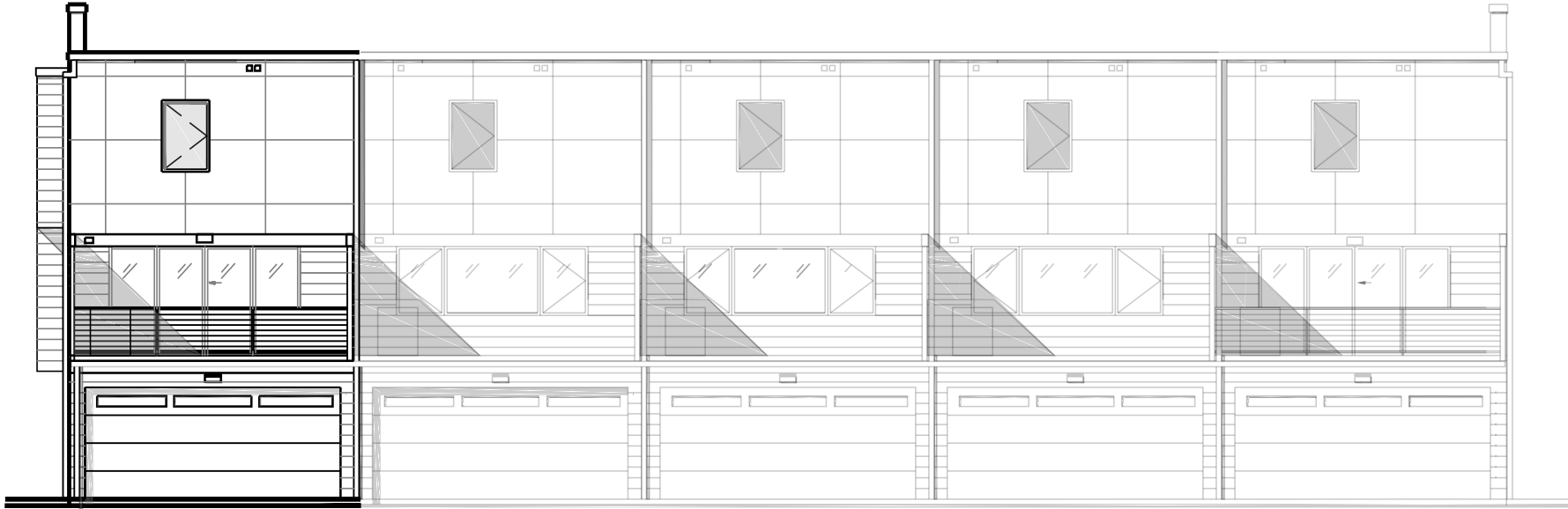
NORTH ELEVATION
