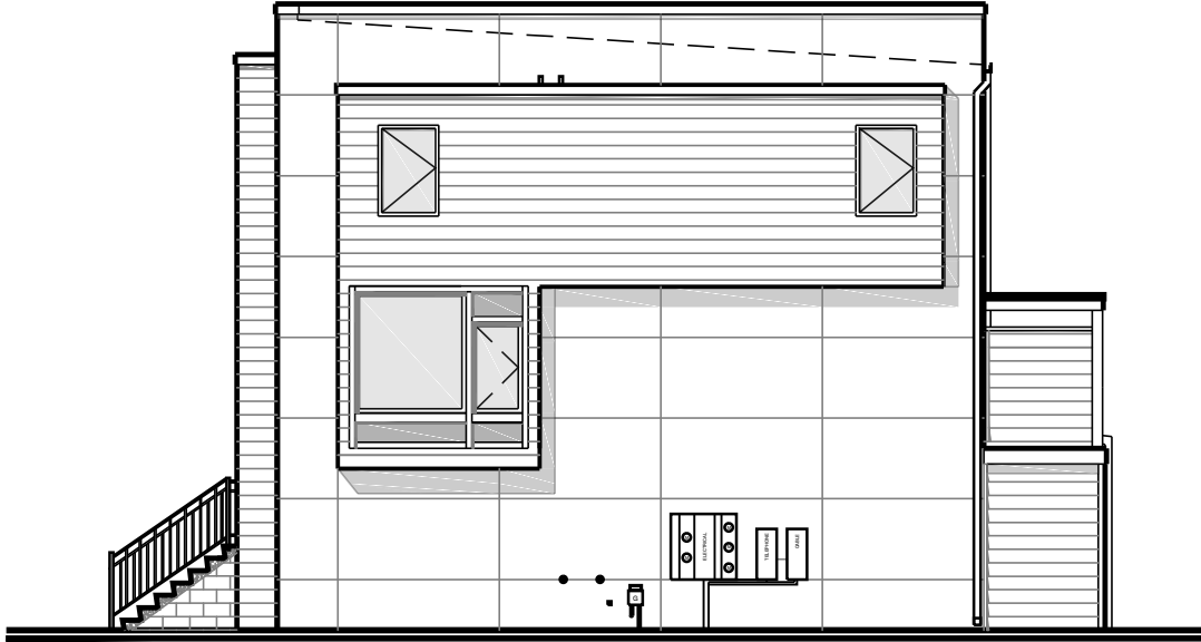
EAST ELEVATION
