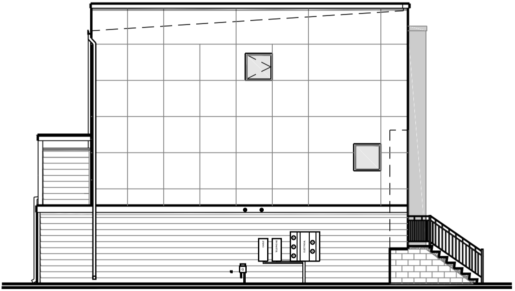
WEST ELEVATION
